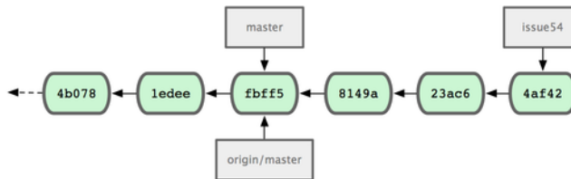
Figure 5.7: L'historique initial de commits de Jessica.
