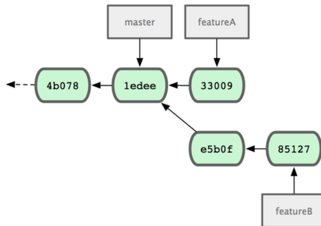
Figure 5.12: L'historique initial de Jessica.
