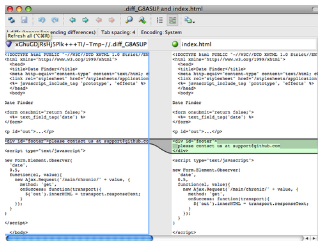
Figure 7.1: P4Merge.
